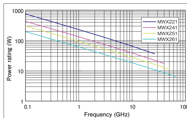
Power rating of MWX2 series at sea level
