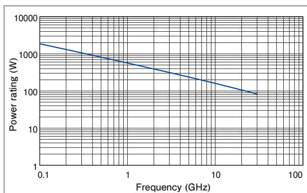
Power rating of MWX1 series at sea level
