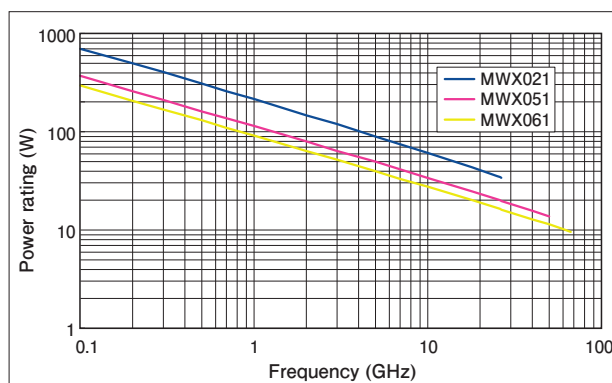
Power rating of MWX0 series at sea level
