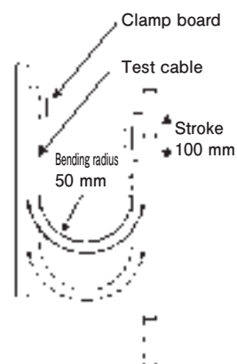
Fig.2 Rolling flex test method
